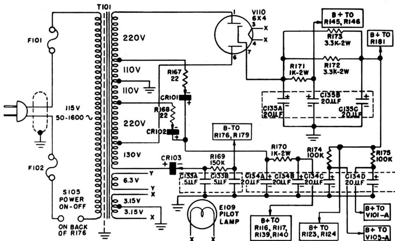
Figure 2-12. Power Supply
