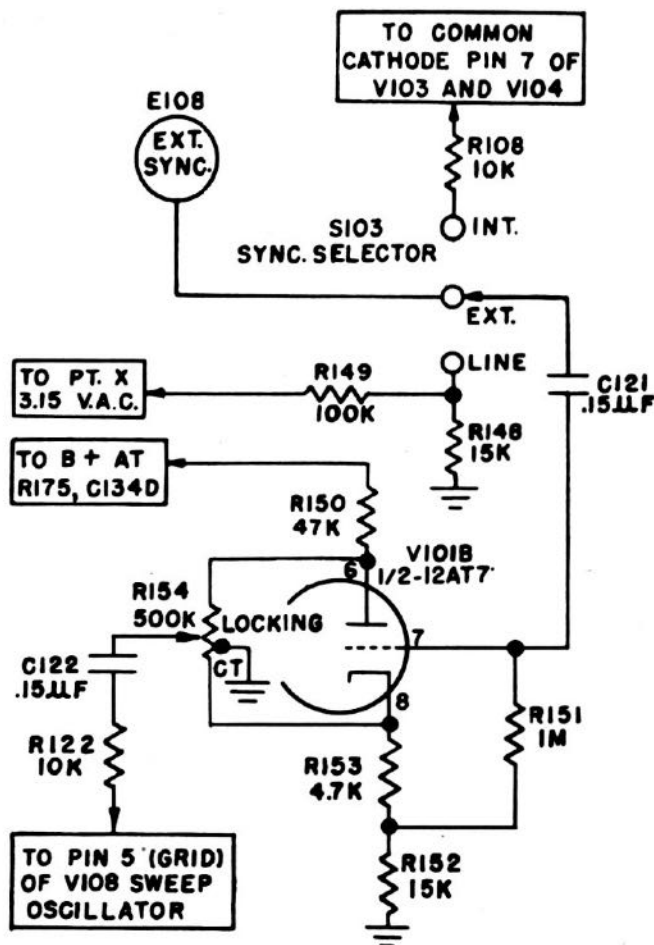
Figure 2-9. Sync. Selector—Amplifier
