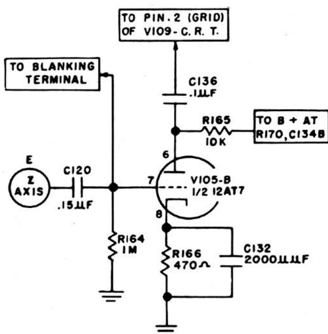
Figure 2-10. Intensity Modulation Amplifier
