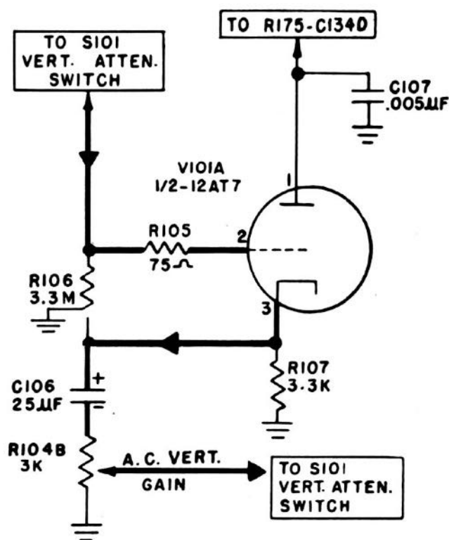
Figure 2-3. Vertical Cathode Follower
