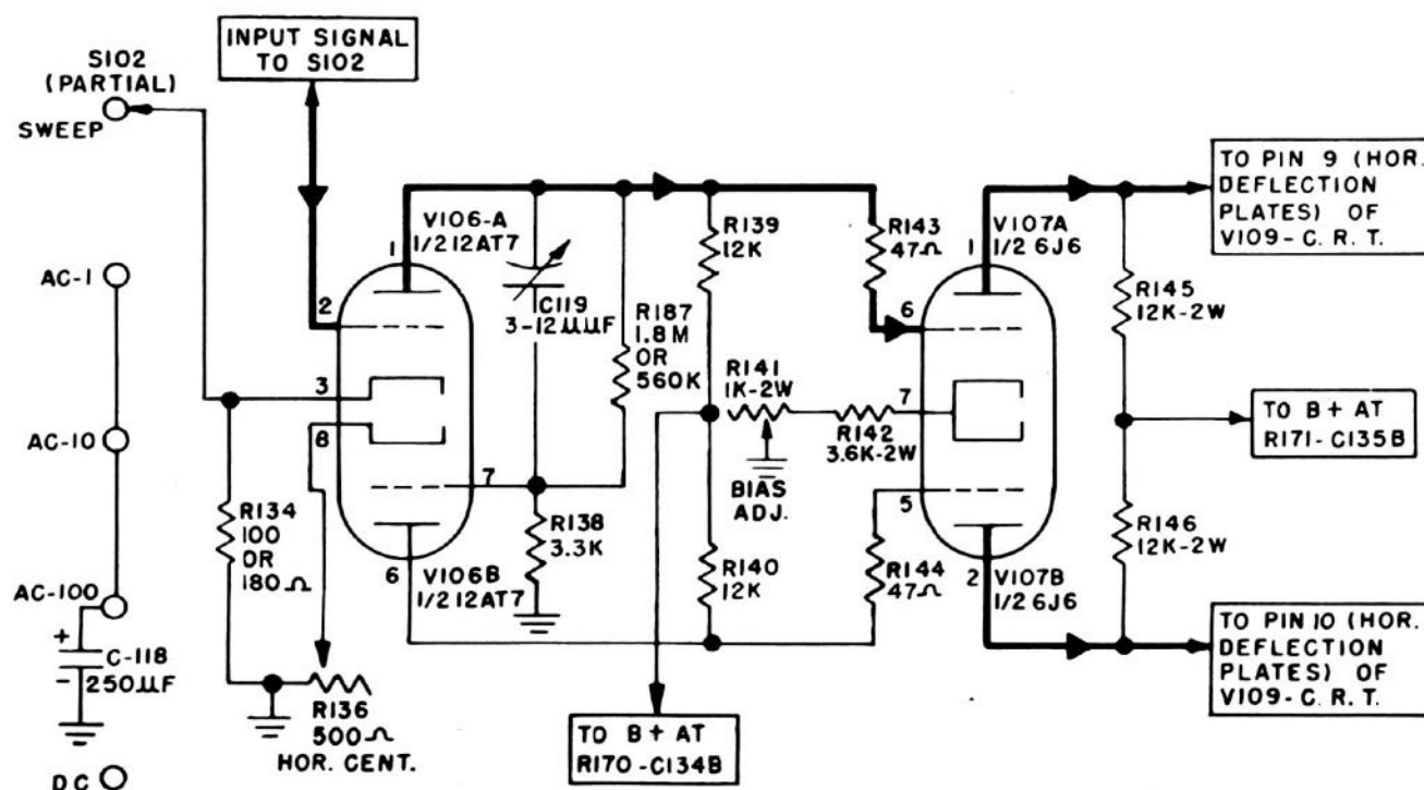
Figure 2-7. Horizontal Amplifiers
