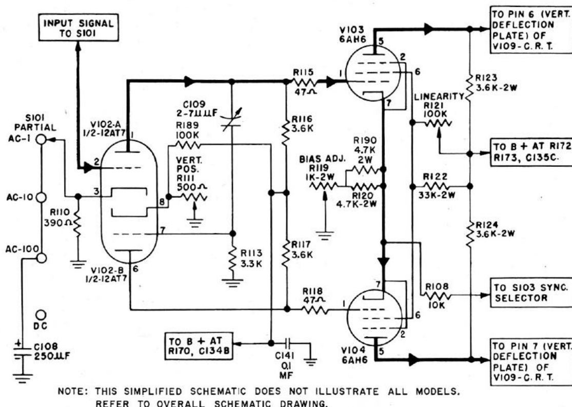
Figure 2-4. Vertical Amplifiers
