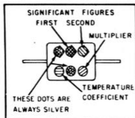
RETMA COLOR CODE FOR TUBULAR CERAMIC- DIELECTRIC CAPACITORS
