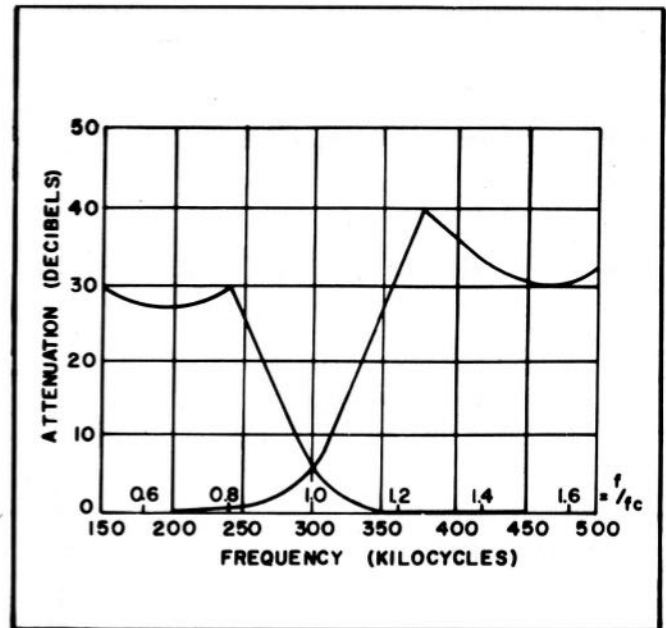
Figure 2-2. Filter Subassembly, Typical Attenuation Characteristics
