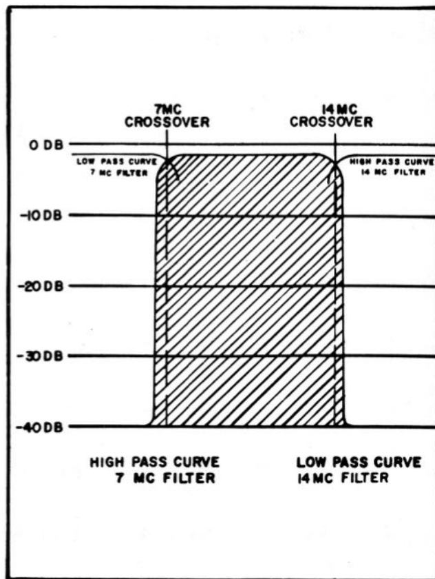
Figure 2-3. Combination of Two Filter Subassemblies, Typical Output at Output Receptacle
