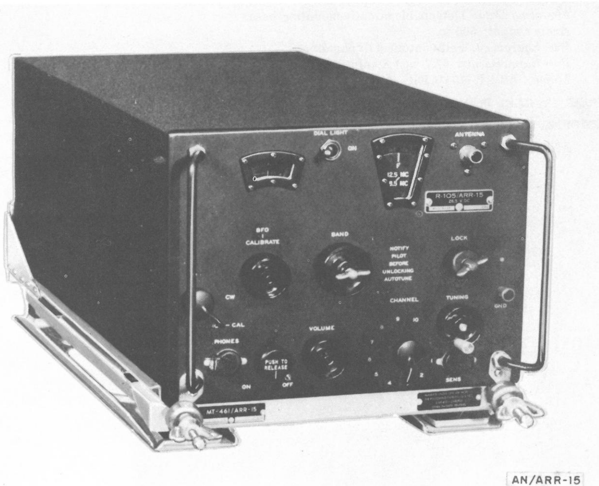
AN/ARR-15
