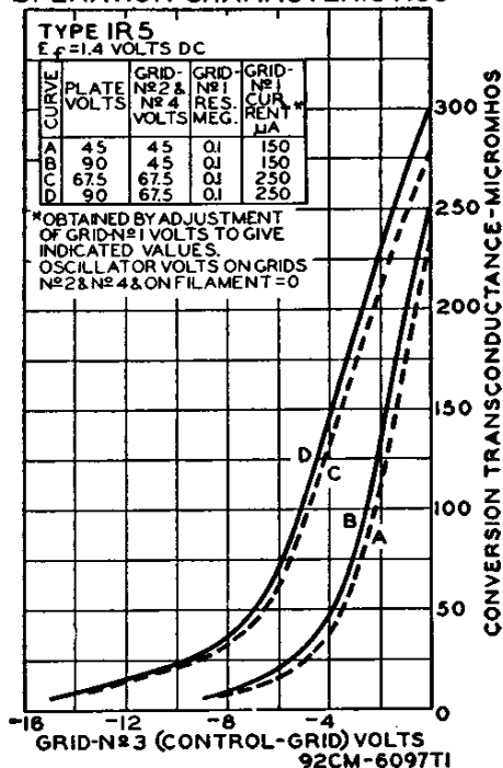
OPERATION CHARACTERISTICS
